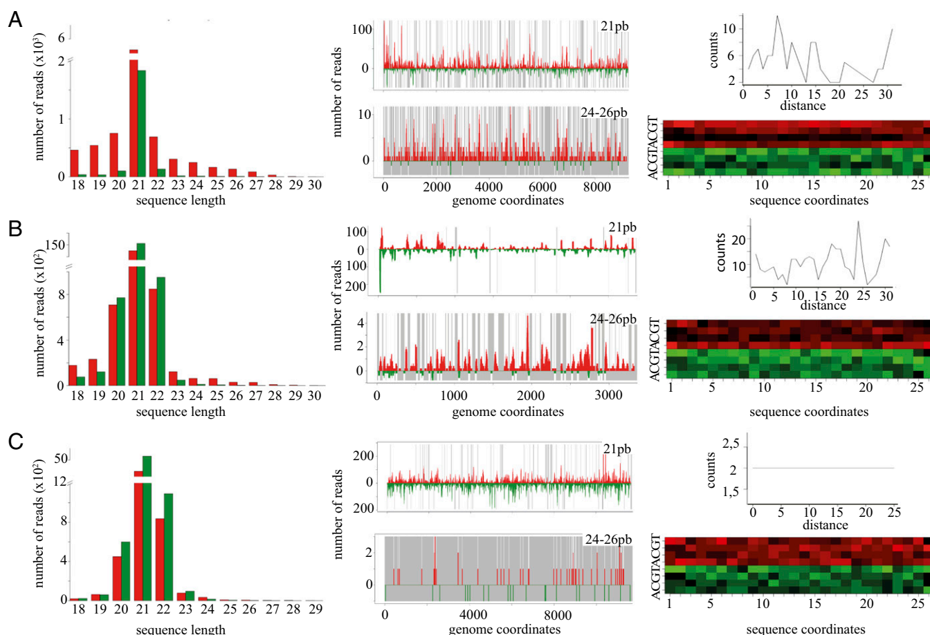
Fig. 3. No viral-derived piRNAs are produced during acute infection of flies. (Left) Size distribution of \beta -eliminated small RNAs extracted from w^{1118} Drosophila infected with DCV (A), DXV segment A (B), and SIN V (C). (Center) Profile of 21 nt and 24–26 nt small viral RNAs that mapped along the viral genome of interest. The sense and antisense small RNAs are shown in red and green, respectively. Uncovered regions are represented as gray lines. (Right) Frequency map of the distance between 24–26 nt small RNAs that mapped to opposite strands of the viral genome. No peak is observed at position 10. The relative nucleotide frequencies per position of the 24–26 nt viral small RNAs that map the sense and antisense of the viral genome are shown in red and green, respectively. The intensity varies in correlation with the frequency. No nucleotide bias (U1 and A10) is observed.
