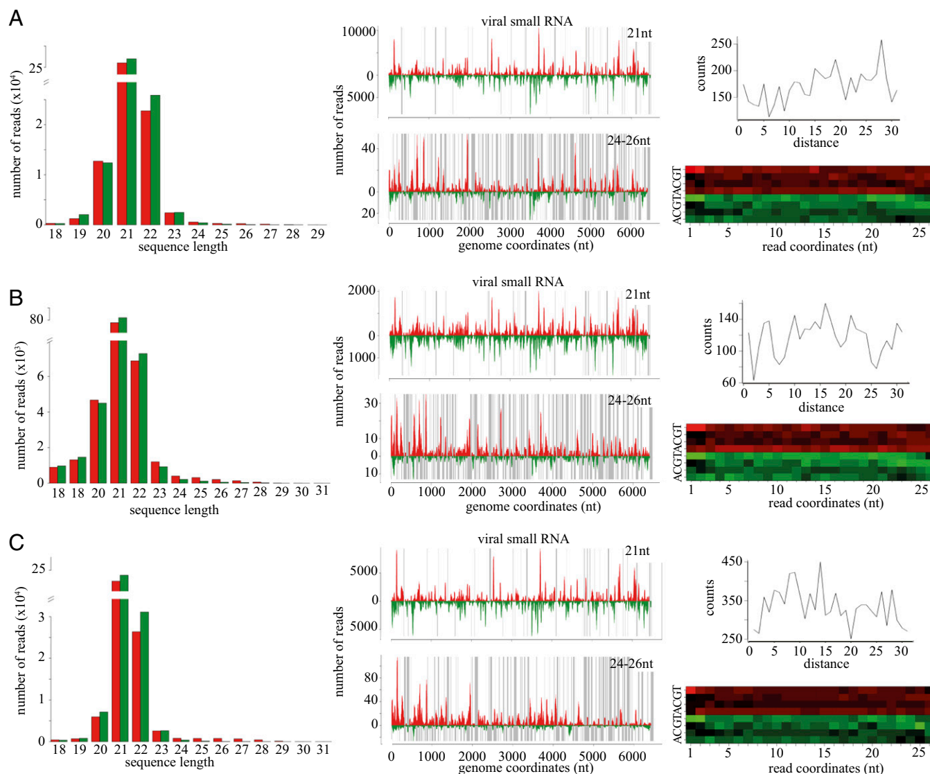
Fig. 5. There is no production of viral-derived piRNAs during Sigma virus infection. (Left) Size distribution of \beta -eliminated small RNAs extracted from Drosophila injected with DmISV. RNA was extracted at 12 dpi for the w 1118 (A) and 22a (B) strains of Drosophila . E320 corresponds to a fly strain persistently infected with DmISV (C). (Center) Profile of 21 nt and 24–26 nt small viral RNA that mapped along the viral genome of interest. The sense and antisense small RNAs are shown in red and green, respectively. Uncovered regions are represented as gray lines. (Right) Frequency map of the distance between 24–26 nt small RNAs that mapped to opposite strands of the viral genome. No peak is observed at position 10. The relative nucleotide frequencies per position of the 24–26 nt viral small RNAs that map the sense and antisense of the viral genome are shown in red and green, respectively. The intensity varies in correlation with the frequency. No nucleotide bias (U1 and A10) is observed.
